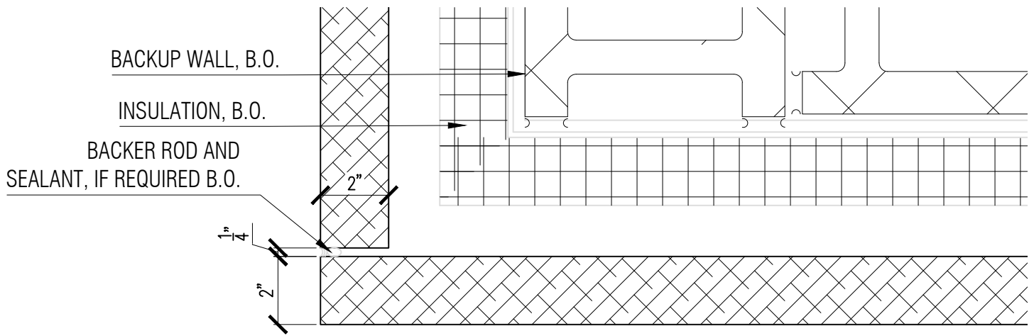
D1 OUTSIDE CORNER WITH BUTT JOINT, 2" THICK STONE
