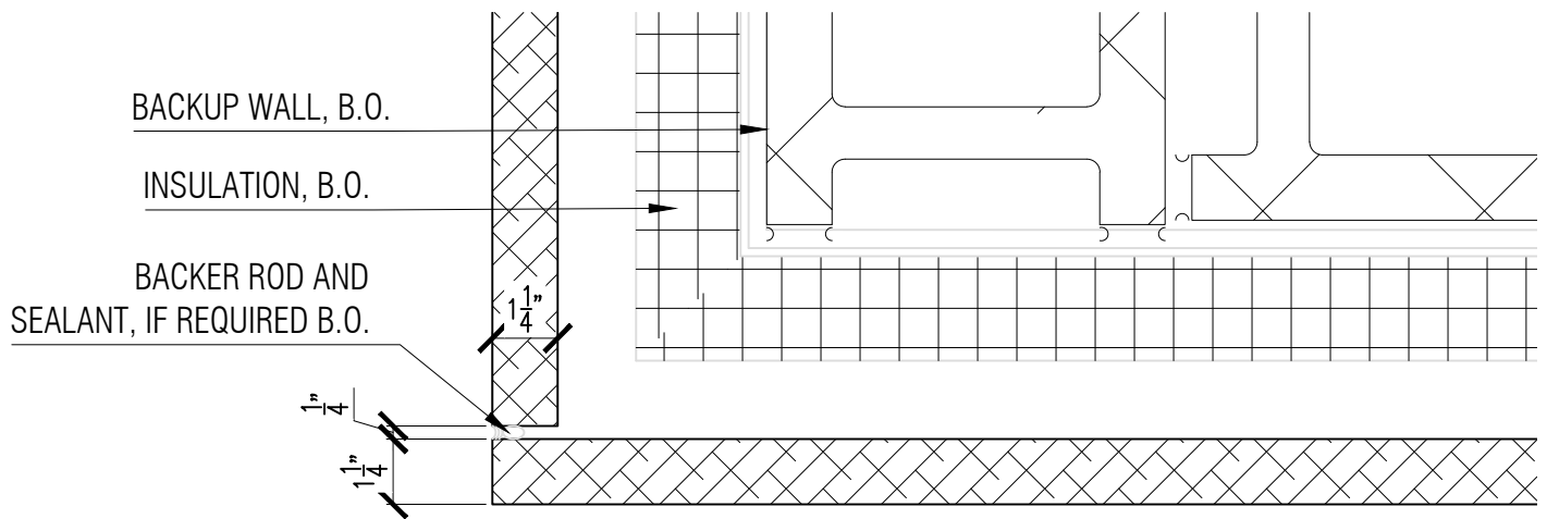
D2 OUTSIDE CORNER WITH BUTT JOINT, 1-1/4" THICK STONE
