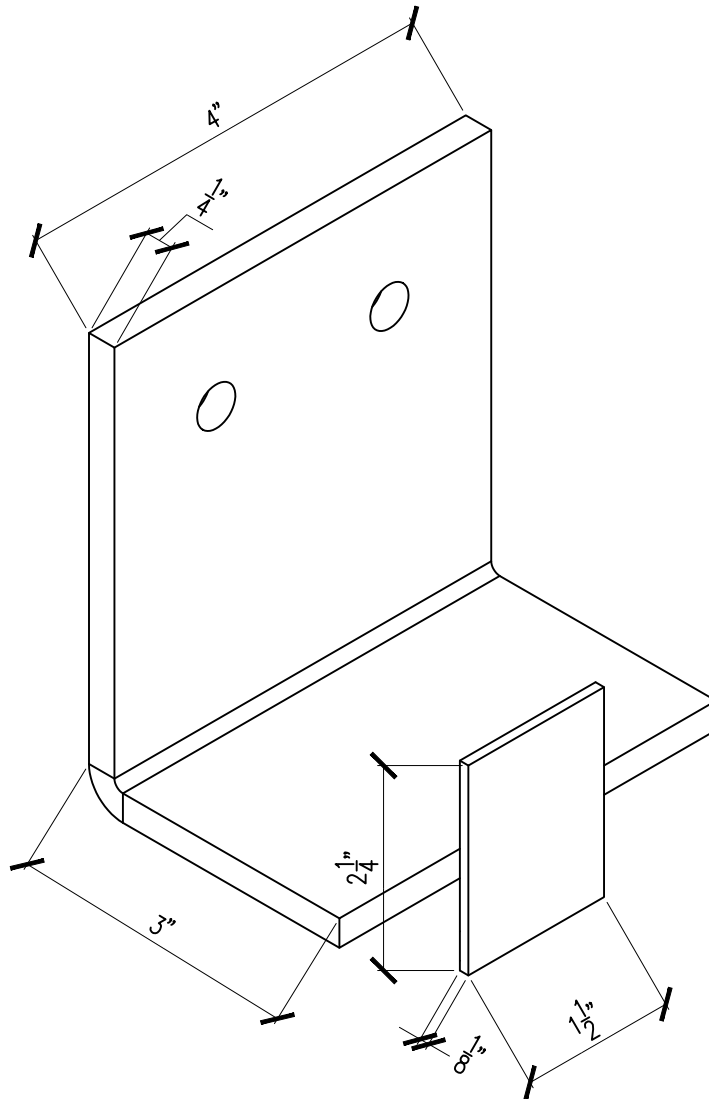
TYPICAL BENT PLATE WITH 1-1/2" x 2-1/4" WELDED TAB
