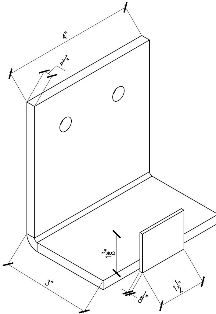
TYPICAL BENT PLATE WITH 1-1/2" x 1-3/8" WELDED TAB
