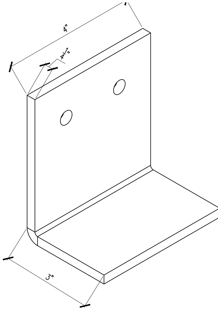
TYPICAL BENT PLATE ANCHOR
