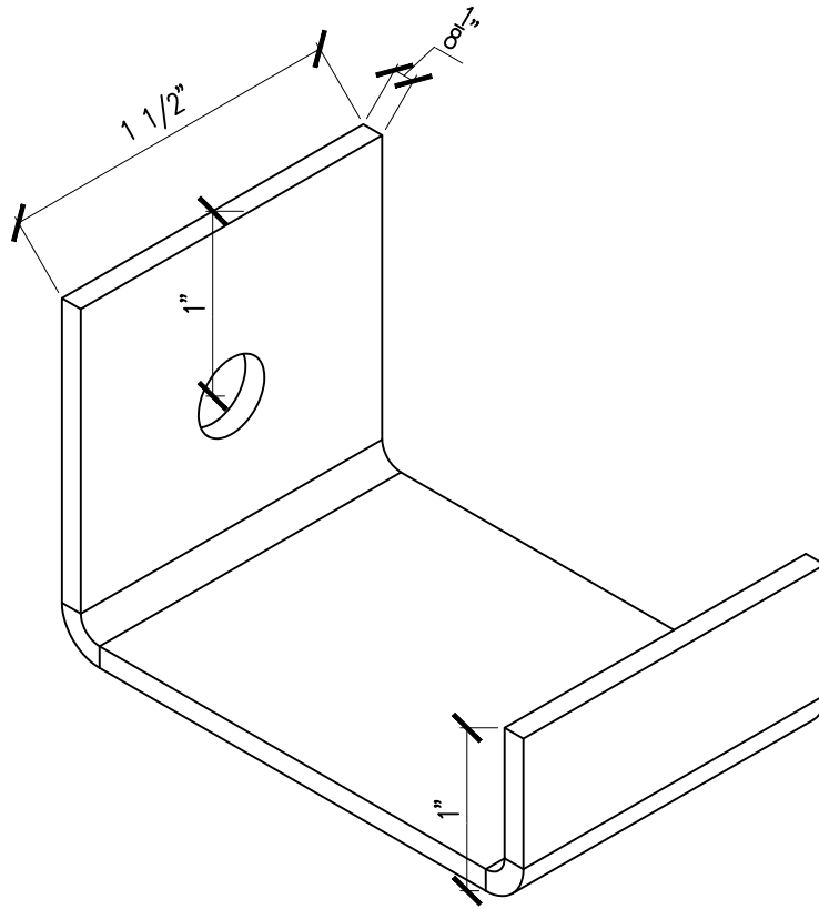
TYPICAL S.S. BENT STRAP ANCHOR
