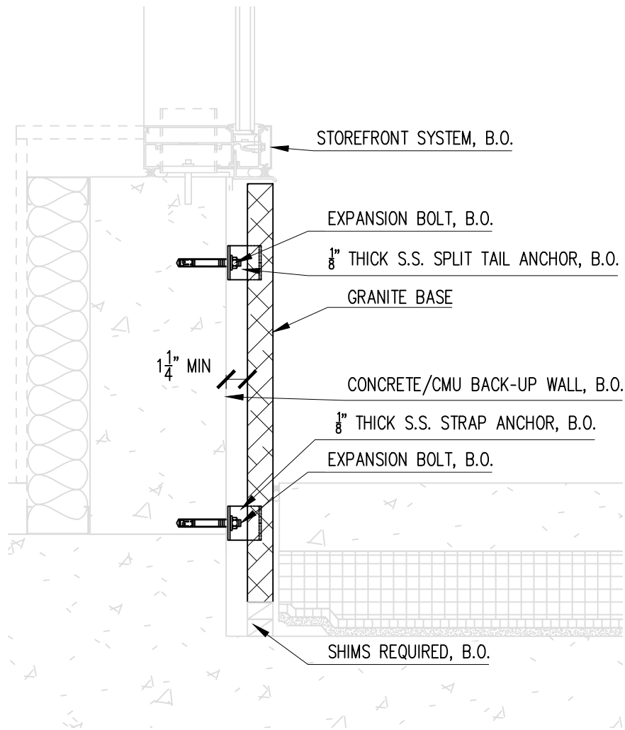
GRANITE BASE WITH SPLIT TAIL ANCHOR, B.O.S IN VERTICAL JOINTS
