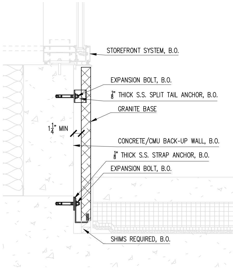
GRANITE BASE WITH STRAP ANCHOR, B.O. BOTTOM, SPLIT TAIL SIDE
