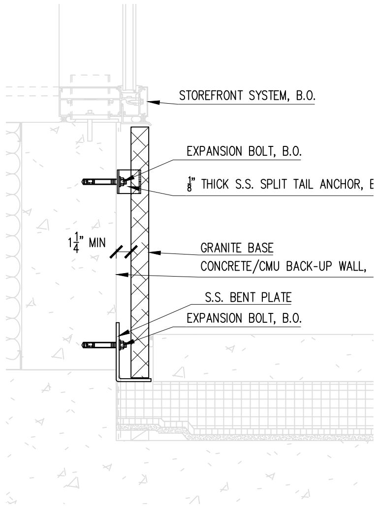
D1 GRANITE BASE WITH BENT PLATE BOTTOM, SPLIT TAIL SIDE
