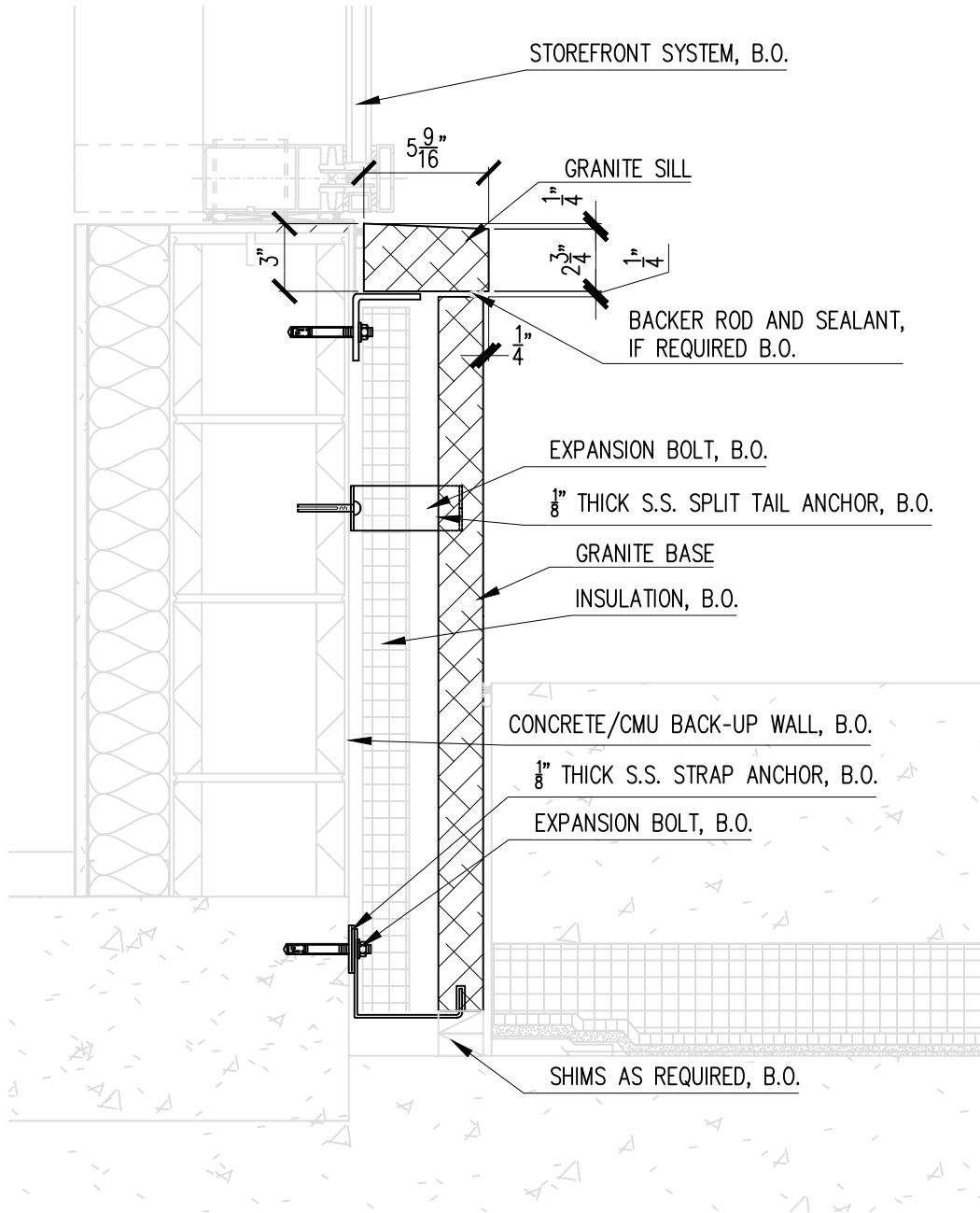
3" THICK SILL WITH SLOPED TOP
