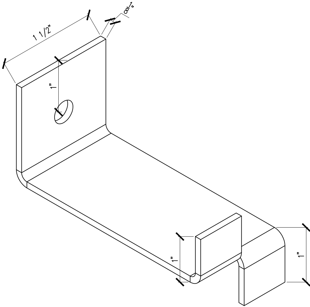
TYPICAL S.S. SPLIT TAIL ANCHOR
