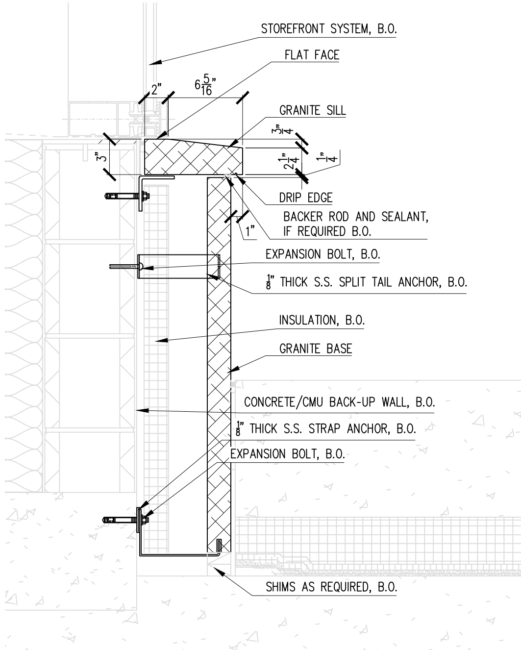
3" THICK FLAT AND SLOPED SILL WITH DRIP EDGE
