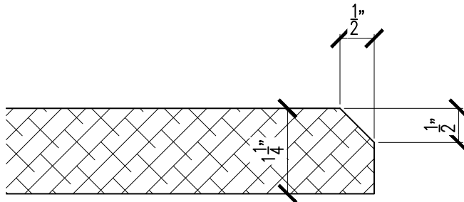
D2 1-1/4" THICK STONE WITH 1/2" X 1/2" CHAMFER
