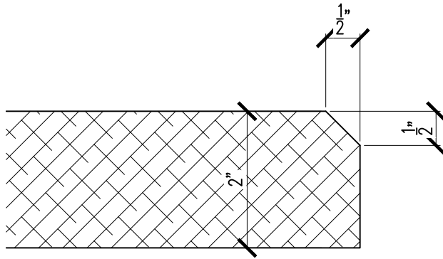
D1 2" THICK STONE WITH 1/2" X 1/2" CHAMFER
